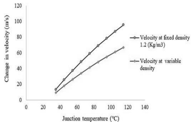
Fig. 1. Change in velocity w. r.t Junction temperature.
