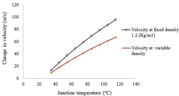
Fig. 5. Change in air velocity with junction temperature.
