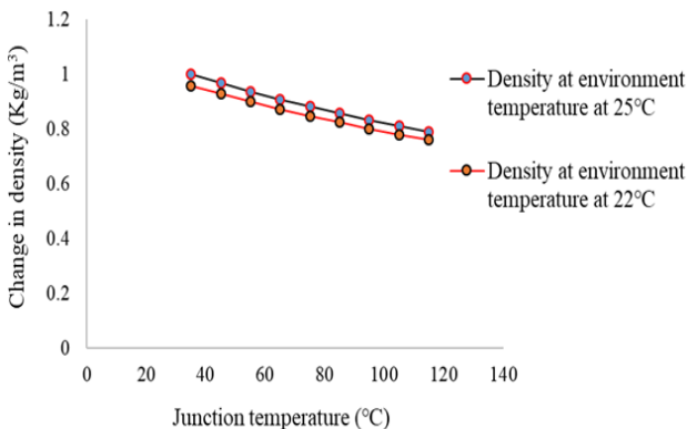
Fig. 3. Change in density with junction temperature.
